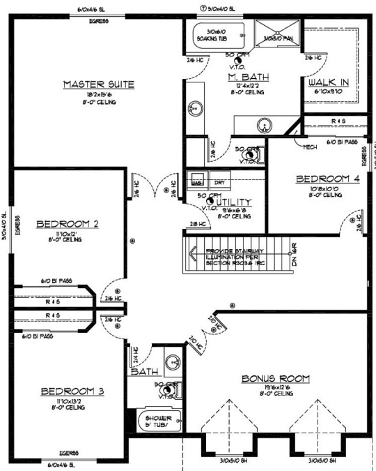
SECOND LEVEL
