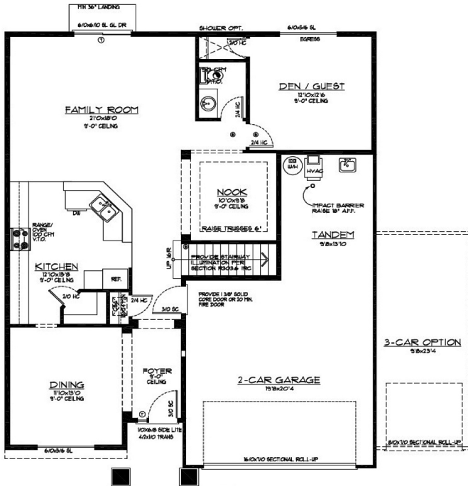
MAIN LEVEL
